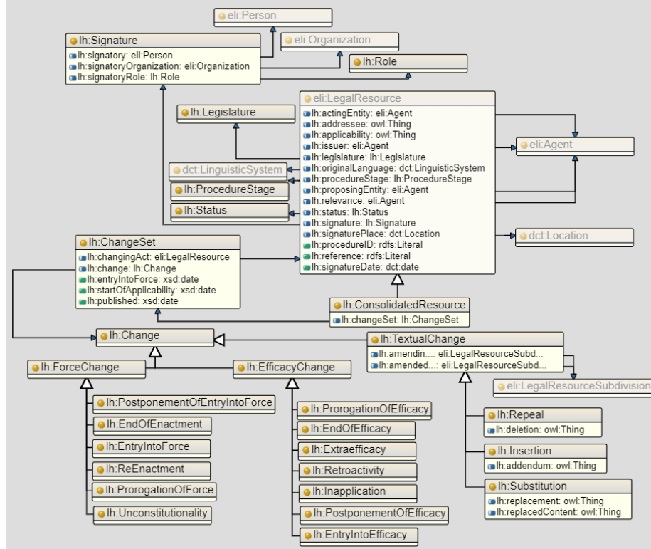
Fig. 2. Class diagram of the LegalHTML Ontology
